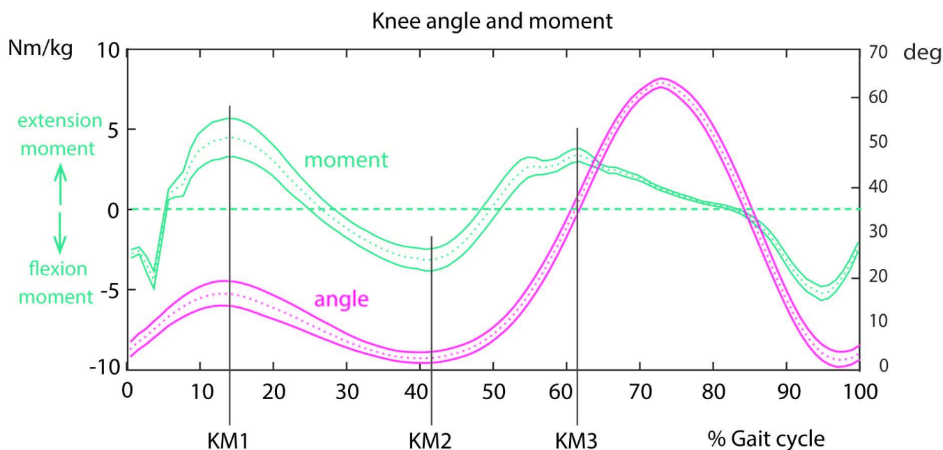
Figure 1. Sagittal knee angle (pink) and moments (green) of HYA during the gait cycle were normalized to the duration of the gait cycle. Maximal knee extension moment at weight acceptance (KM1), maximal flexion moment during mid-stance (KM2) and maximal extension moment around push-off (KM3) were identified. Moments and angles around knee, hip and ankle were also evaluated at these instants.
